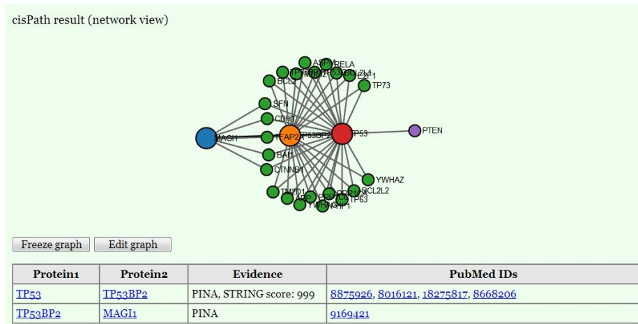
Figure 1: networkView result
