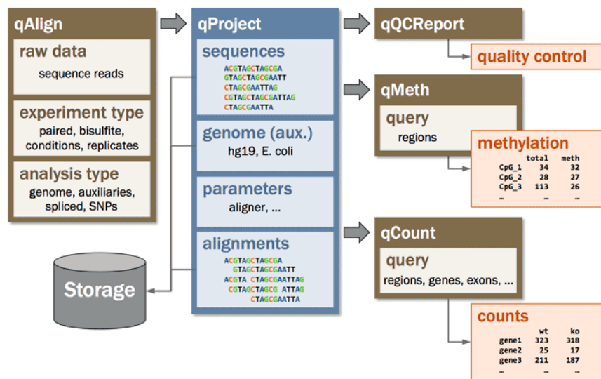
Figure 1: QuasR package overview
