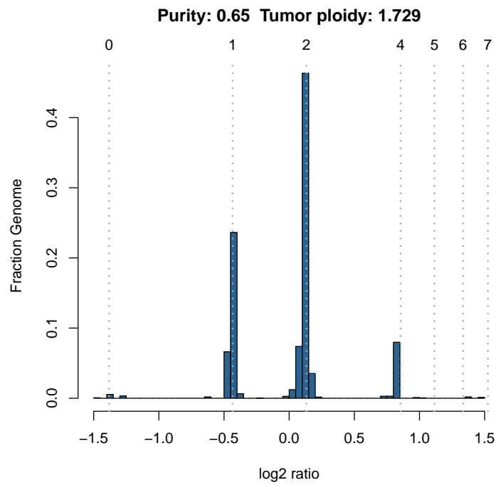
Figure 3: Log-ratio histogram.
