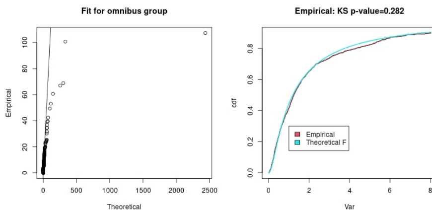
Figure 11: An output from the anota2seqPerformQC function (used with parameter useRVM = TRUE ) comparing obtained variances to the theoretical F-distribution
