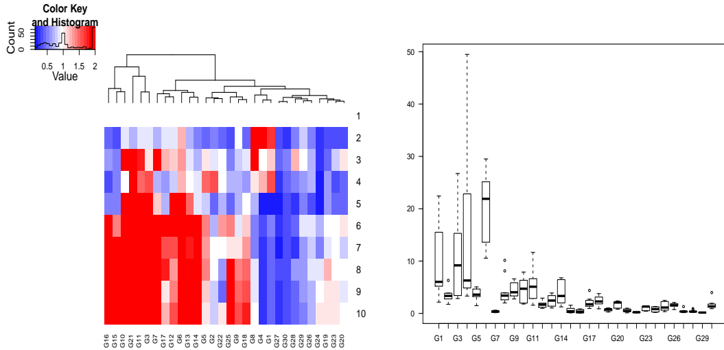
Figure 2: Barcode and boxplot using default parameters, spreading in the color key is not well balanced (see histogram)
