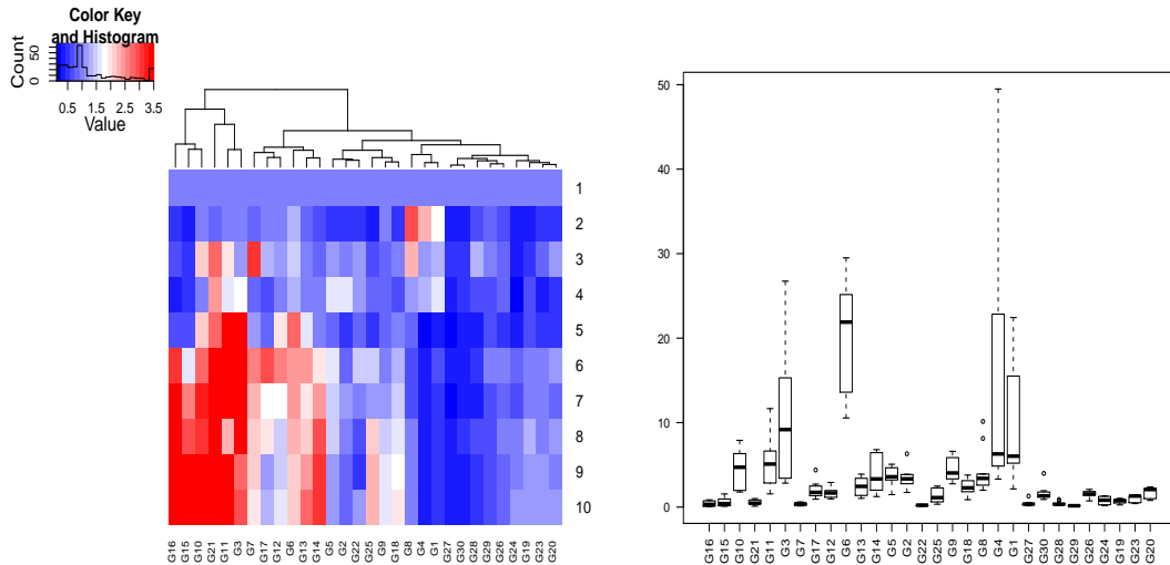
Figure 5: Using values normalized by method "first", same changes as described in Figure 4
