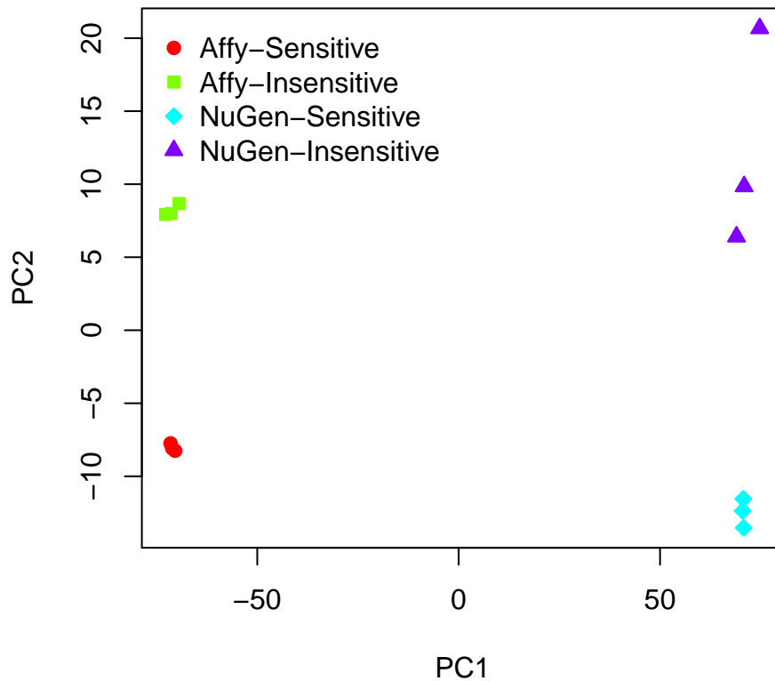
Figure 3: PCA plot
