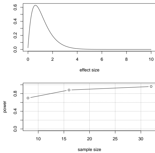
Figure 6: Estimated density of effect sizes and predicted power curve for the deepSAGE experiment.
