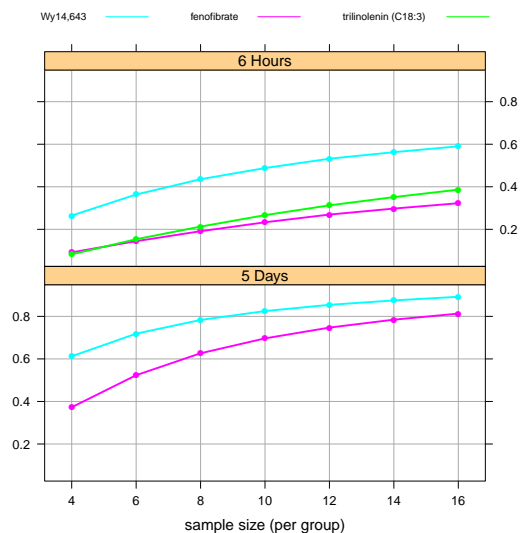
Figure 5: Predicted power curves for the nutrigenomics experiment.
