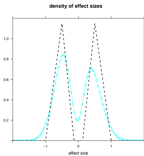
Figure 8: Estimated density and true (bitriangular) density of effect sizes using Tikhonov regularization.
