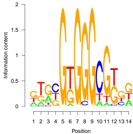
(b) Dme-FFS-sr_SANGER_5_FBgn0003499
